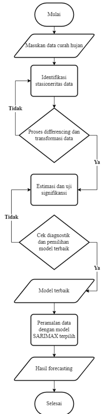
Gambar 2 Flowchart forecasting model SARIMAX
